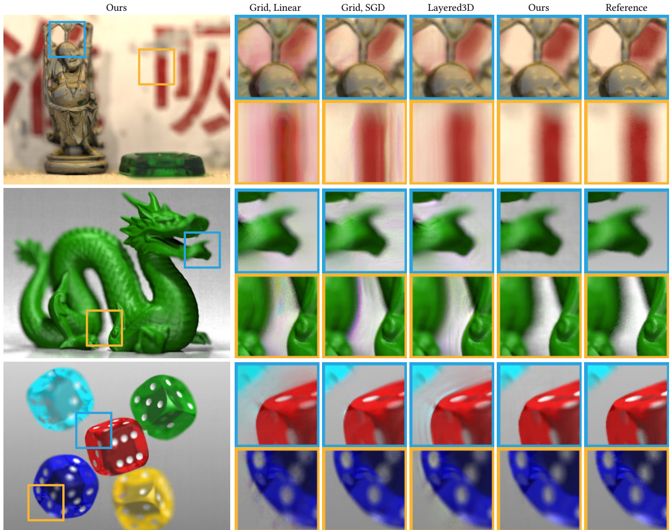
Fig. 4. Quality comparison between our, Layered3D and grid-based approach on the Buddha , Green Dragon , and Dice scene. Note that, for Ours , we demonstrate a test view that is not part of the training dataset. For the grid-based approach, we show results obtained by the linear and the SGD solver, respectively. More details are in Section 6.3. See also the supplemental for more results with GIF animations and rendered high-resolution views.
